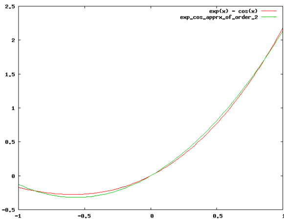
Fig. 5. Approximating \exp(x) - \cos(x) using Chebyshev
