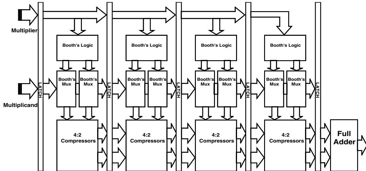
Figure 11. Multiplier Datapath Structure
