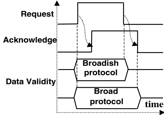
Figure 1. Four-phase Handshake Protocols
