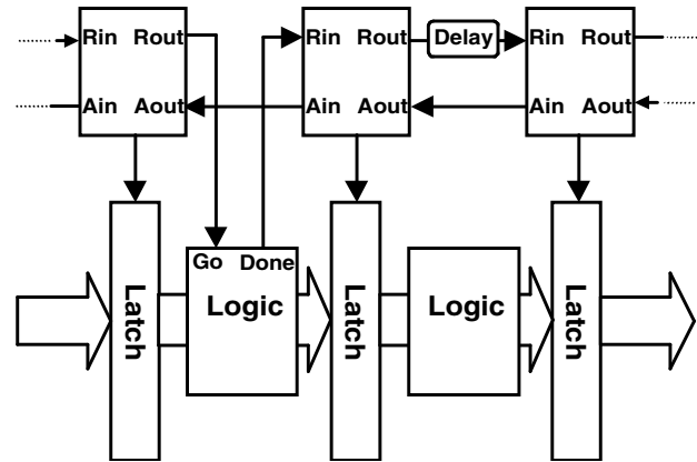
Figure 2. Asynchronous Pipeline with Processing
