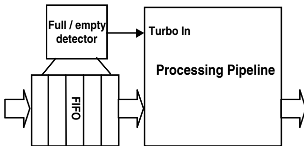
Figure 10. Controlling the Turbo Input According to Demand
