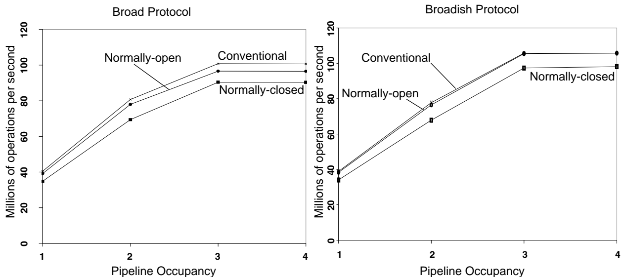
Figure 12. Plot of Throughput Against Pipeline Occupancy for Latch Controller Designs
