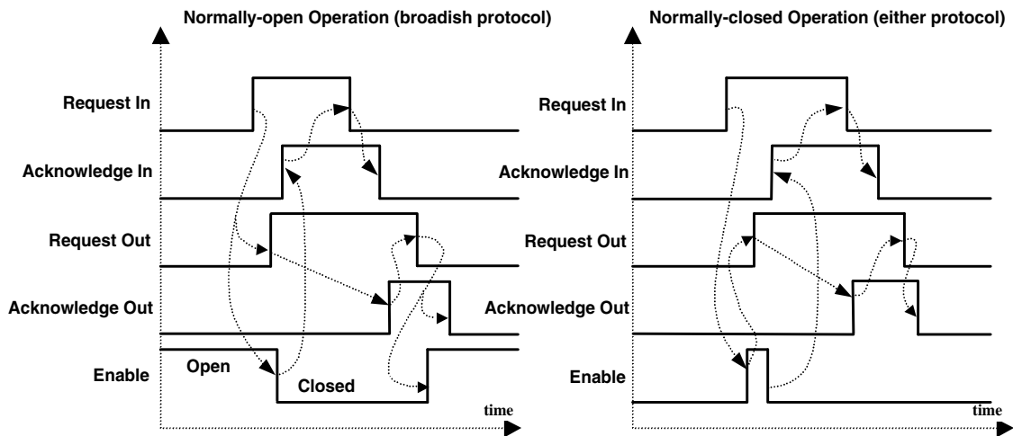
Figure 3. Latch Controller Operating Modes
