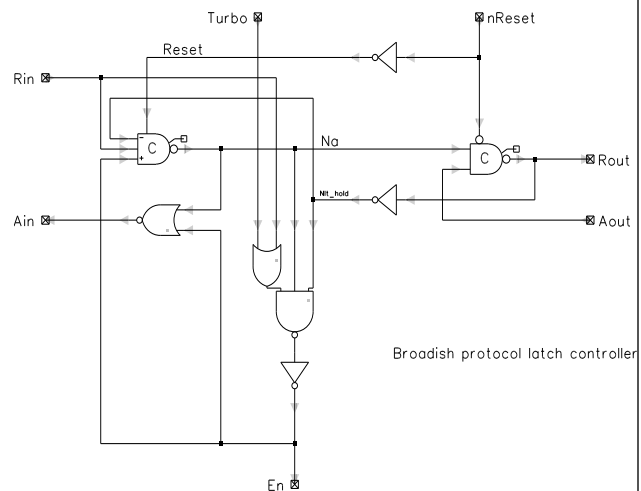
Figure 5. Broadish Protocol Reconfigurable Latch Controller
