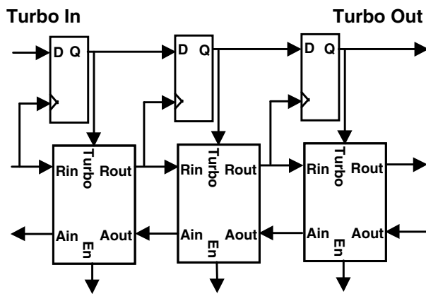
Figure 9. Modified Pipeline with Turbo Signal
