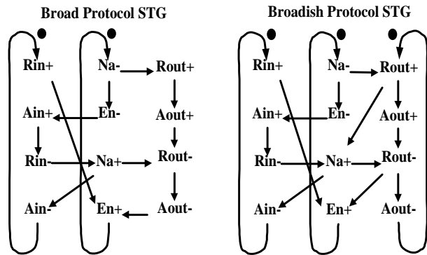
Figure 8. Broad and Broadish Protocol STGs for Normally-Closed Operation
