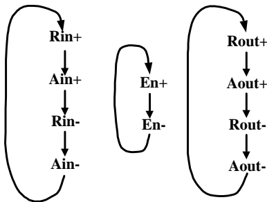
Figure 6. Latch Controller Cycles
