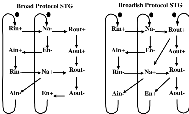
Figure 7. Broad and Broadish Protocol STGs for Normally-Open Operation
