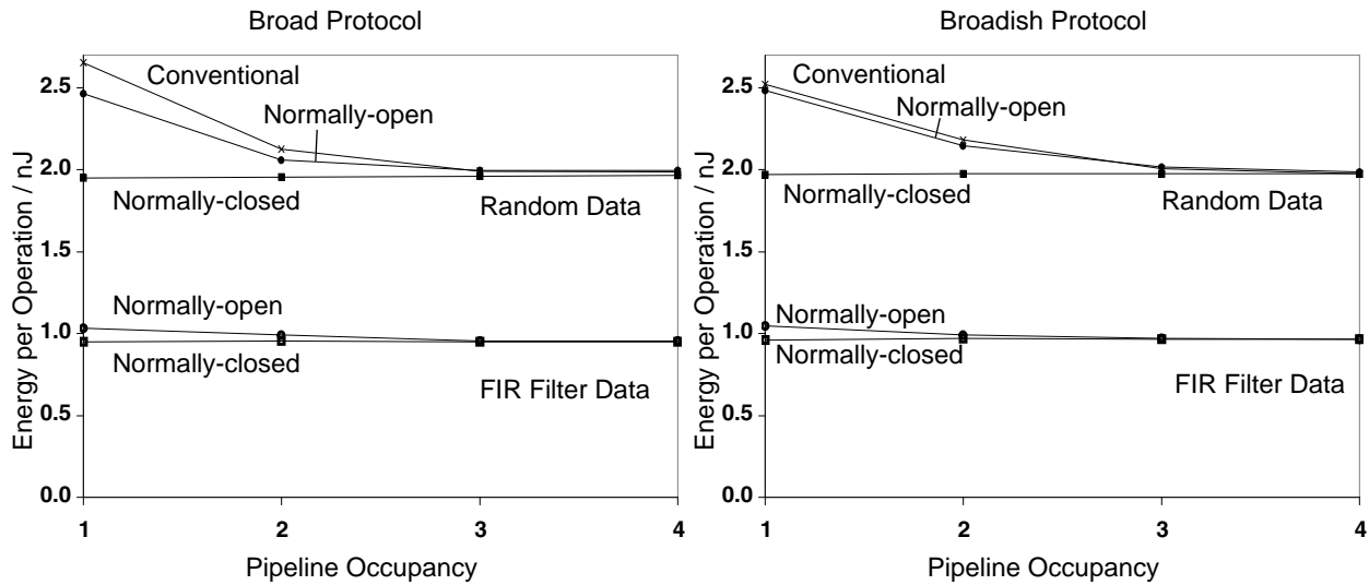
Figure 13. Energy per Operation Against Pipeline Occupancy for Latch Controller Designs
