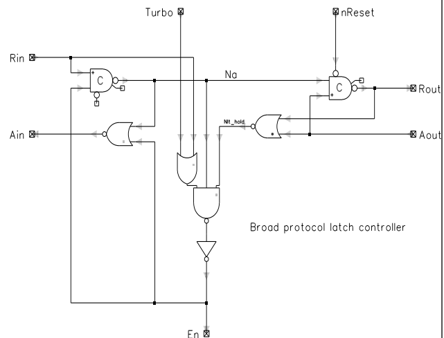
Figure 4. Broad Protocol Reconfigurable Latch Controller
